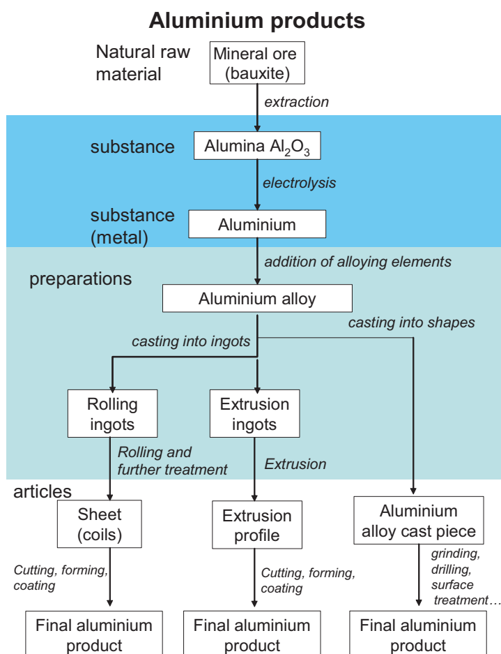
Figure 7 Example of the general transition point from mineral to final aluminium article 45
